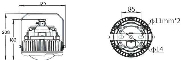
Dimension ( mm )
