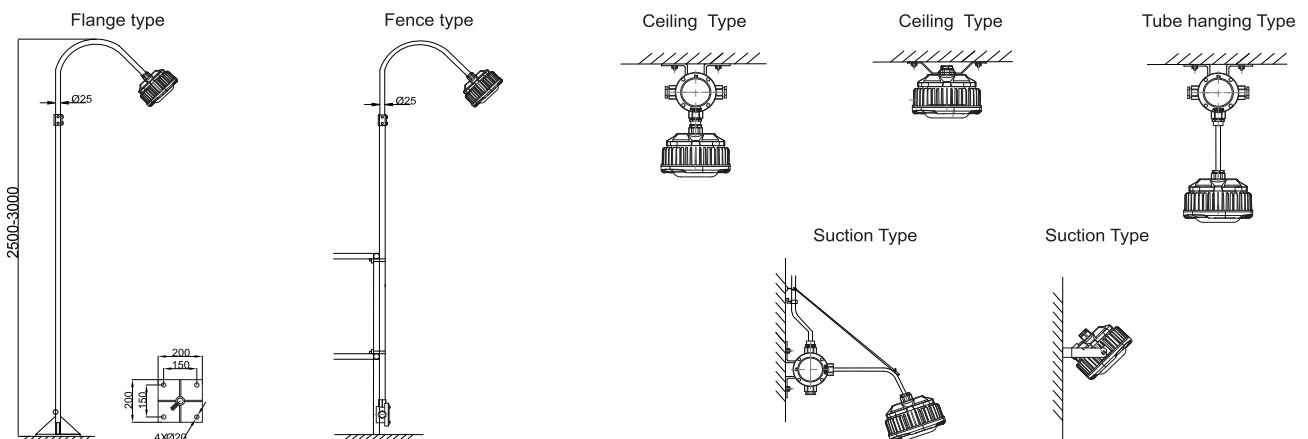
Installation Mode
