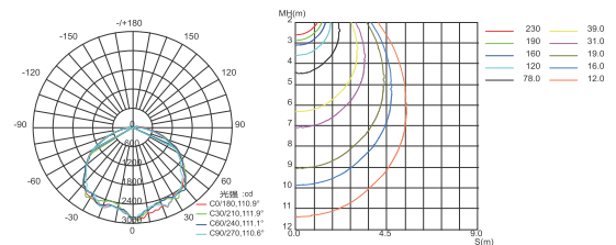
Light Distribution Curve
